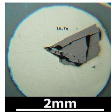
Polished tellurium in T100-52 mount
